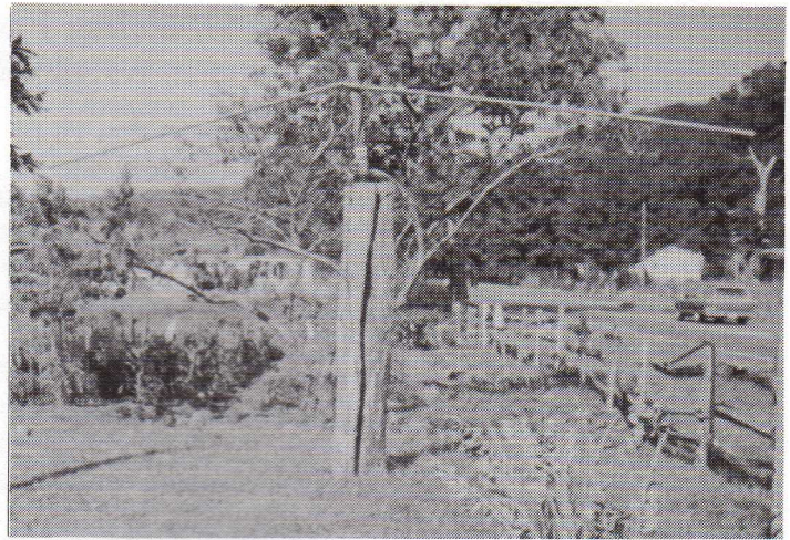
15 meter antenna at the QTH of Richard Maxham, W8INP, Monterey, Virginia. "A neighbor asked if this was an elaborate watering system for the garden!"
